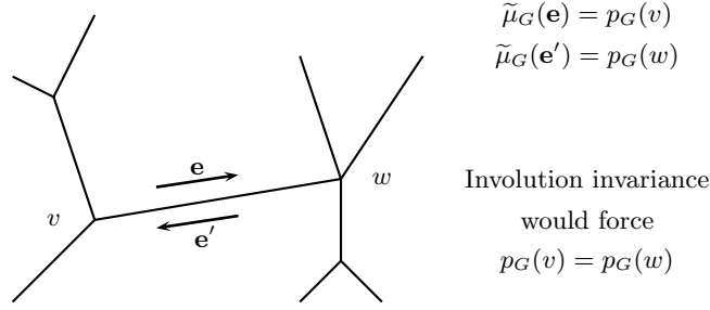
Fig. 8. Given G = (V, E) we let p_G(v) denote the probability that v is the root of G , and if \tilde{\mu} is the induced measure, we write \tilde{\mu}_G for the marginal measure given G . For any directed edge (v, w) of G , the measure \tilde{\mu}_G puts mass p_G(v) on the edge (v, w) and puts mass p_G(w) on the edge (w, v) . If one has involution invariance, then \tilde{\mu}_G(v, w) = \tilde{\mu}_G(w, v) , and we see that p_G(v) = p_G(w) . Thus, p_G(\cdot) is constant on each connected component of G whenever one has involution invariance.
