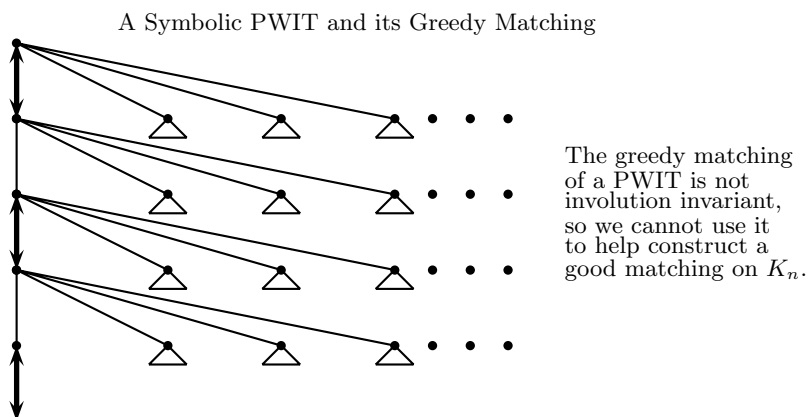
Fig. 7. To construct the greedy matching of a PWIT one takes the shortest edge e out of the root, removes all of the vertices incident to e , and proceeds recursively. The expected cost per vertex of the greedy matching is equal to one-half, which beats the unbeatable limiting average cost of \zeta(2)/2 per vertex for K_n .
