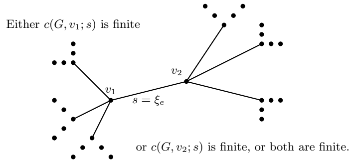
Fig. 6. The edge e = (v_1, v_2) of G is in the minimal spanning forest if and only if at least one of the trees c(G, v_1; s) and c(G, v_2; s) is finite when s = \xi_e .
