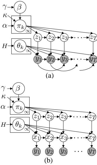
Fig. 1. Sticky HDP-HMM prior on (a) switching VAR(2) and (b) SLDS processes with the mode evolving as z_{t+1} | \{\pi_k\}_{k=1}^{\infty}, z_t \sim \pi_{z_t} for \pi_k | \alpha, \kappa, \beta \sim \text{DP}(\alpha + \kappa, (\alpha\beta + \kappa\delta_k)/(\alpha + \kappa)) . Here, \beta | \gamma \sim \text{GEM}(\gamma) and \theta_k | H \sim H . The dynamical processes are as in Table I.
