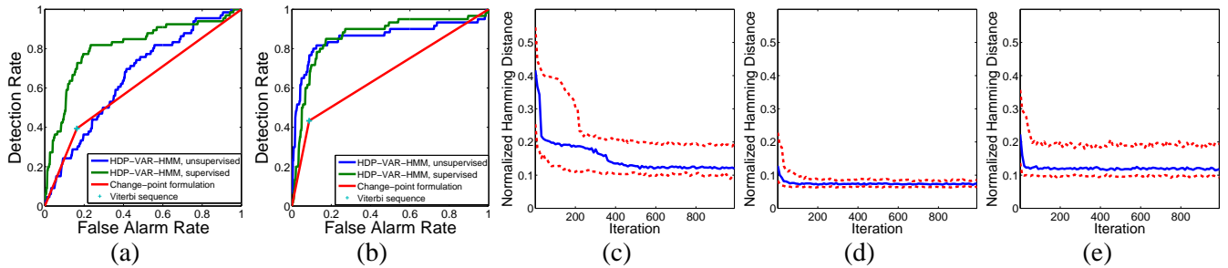
Fig. 5. (a)-(b) ROC curves for the unsupervised HDP-VAR-HMM, partially supervised HDP-VAR-HMM, and change-point formulation of [15] using the Viterbi sequence for segmenting datasets 1-3 and 4-6, respectively. (c)-(e) The 10th, 50th, and 90th Hamming distance quantiles over 100 trials are shown for sequences 4, 5, and 6, respectively.
