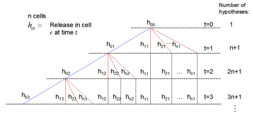
Fig. 1. Hypothesis tree for a region with n cells at time step 3. Hypothesis h_{ct} represents a release in cell c at time t .
