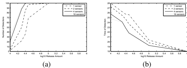
Fig. 2. (a) Number of detections per 100 simulation data sets and (b) time to first detection versus release amount. Actual release time was 16 seconds.
