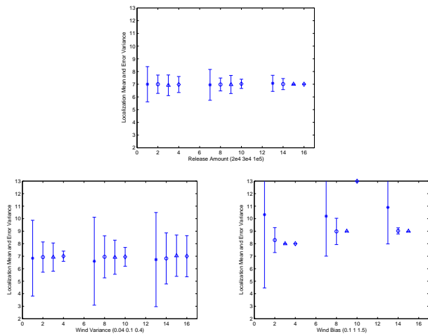
Fig. 4. Localization mean and error variance of 4 and 16 sensors at time of first detection ( * and o ) and after accruing information ( \Delta and \diamond ) for three values of release amount (top), unmodeled wind variance (bottom left), and unmodeled wind bias (bottom right).
