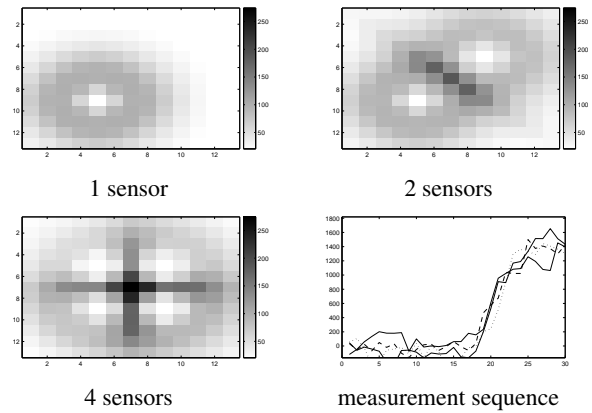
Fig. 3. Maximum likelihood ratio at every cell in region of interest for 1,2, and 4 sensor configuration. The measurement sequence for the 4 sensor configuration sequence is also shown.
