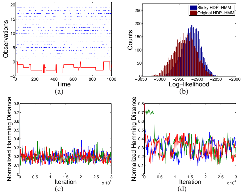
FIG 8. (a) Observation sequence (blue) and true state sequence (red) for a five-state HMM with multinomial observations. (b) Histogram of the predictive probability of test sequences using the inferred parameters sampled every 100 th iteration from Gibbs iterations 10,000 to 30,000 for the sticky and original HDP-HMM. The Hamming distances over 30,000 Gibbs samples from three chains are shown for the (c) sticky HDP-HMM and (d) original HDP-HMM.
