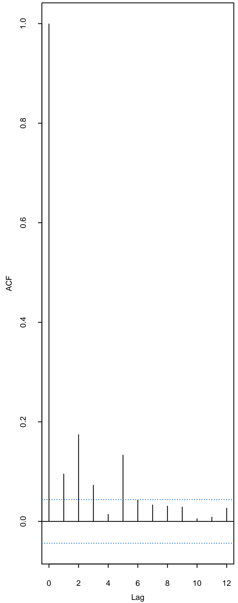
Series : ford.s^2
