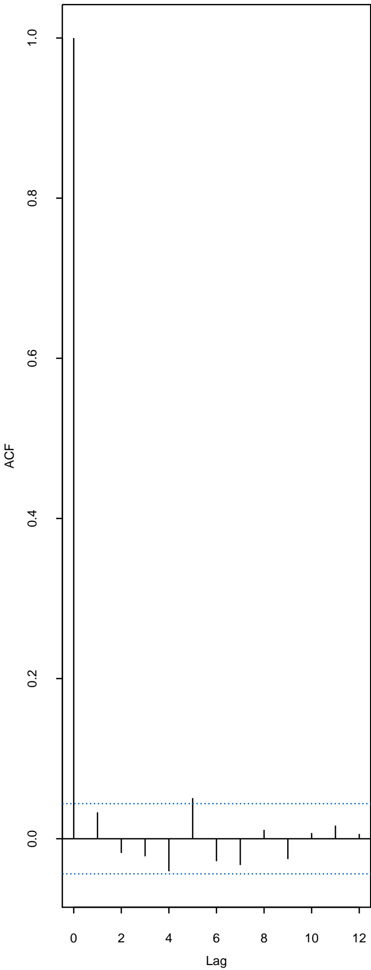
Series : ford.s
