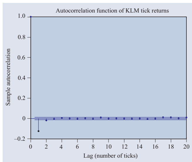
Figure 7. Autocorrelation function of tick by tick returns on KLM shares traded on the NYSE. Time scale: ticks.
