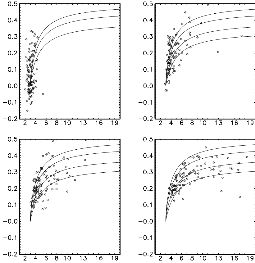
Figure 4: Combinations of the first-order autocorrelation of squared observations and kurtosis for the GARCH(1,1) model with normal errors for various values of \alpha + \beta together with 100 realizations based on T simulated observations from an IGARCH(1,1) model with \alpha_0 = \alpha = 0.1 : T = 100 (first panel), 500 (second panel), 1000 (third panel) and 2000 (fourth panel). Isoquants from lowest to highest: \alpha + \beta = 0.999, 0.99, 0.95 and 0.9 .
