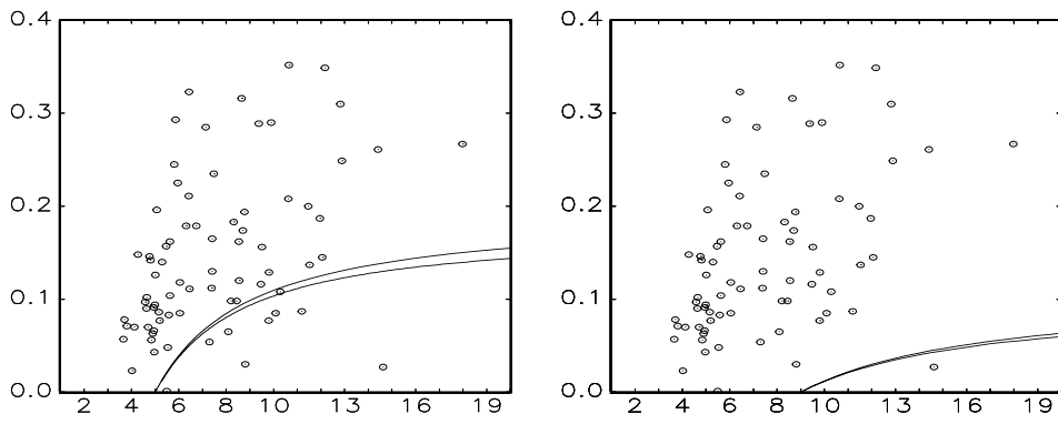
Figure 8: Combinations of the first-order autocorrelation of squared observations and kurtosis for the ARSV(1) model with t-distributed errors for various values of \beta : left panel: t(7) , right panel: t(5) . Isoquants from lowest to highest: \alpha + \beta = 0.99 and 0.95 . The observed combinations are the same as in the lower-right panel of Figure 1.
