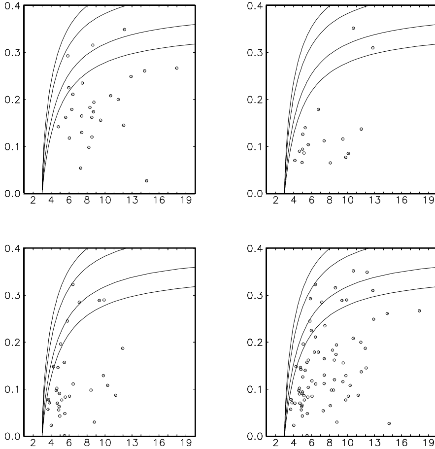
Figure 3: Combinations of the first-order autocorrelation of squared observations and kurtosis for the GARCH(1,1) model with normal errors for various values of \alpha + \beta together with observed combinations of daily rates of return: Upper-left panel, daily returns of the 27 most traded stocks at the Stockholm Stock Exchange. Lower-left panel, the S&P 500 index 3 January 1928 to 19 September 2001, divided to 20 equally long subseries. Upper-right panel, five major daily exchange rates series divided to 34 subseries. Lower-right panel, all observations. Isoquants from lowest to highest: \alpha + \beta = 0.999, 0.99, 0.95 and 0.9 .
