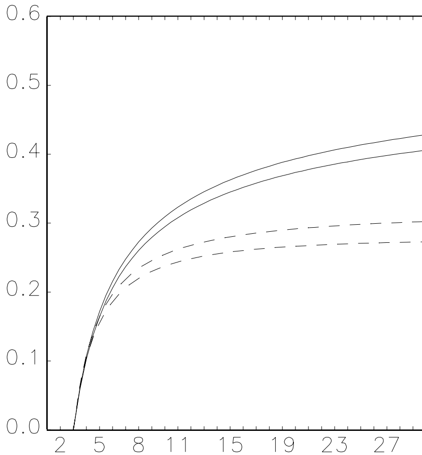
Figure 11: Combinations of two first-order autocorrelations, the squared observations (dashed line) and the absolute observations (solid line), and corresponding kurtosis values for the ARSV(1) model with normal errors for \beta = 0.95 (low) and \beta = 0.99 (high).
