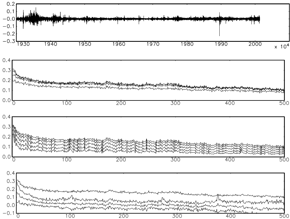
Figure 1: Uppermost panel, log-returns of the S&P 500 index 3 January 1928 to 19 September 2001. Second panel, the autocorrelation function of |r_t|^m , m = 0.25, 0.5, 0.75, 1 , from low to high, for the S&P 500 index. Third panel, the autocorrelation function of |r_t|^m , m = 1, 1.25, 1.5, 1.75, 2 , from high to low, for the S&P 500 index. Lowest panel, the autocorrelation function of |r_t| for the whole series (highest graph) and the mean of the corresponding autocorrelations of the 20 equally long subseries of the S&P 500 index together with the plus/minus one standard deviation band.
