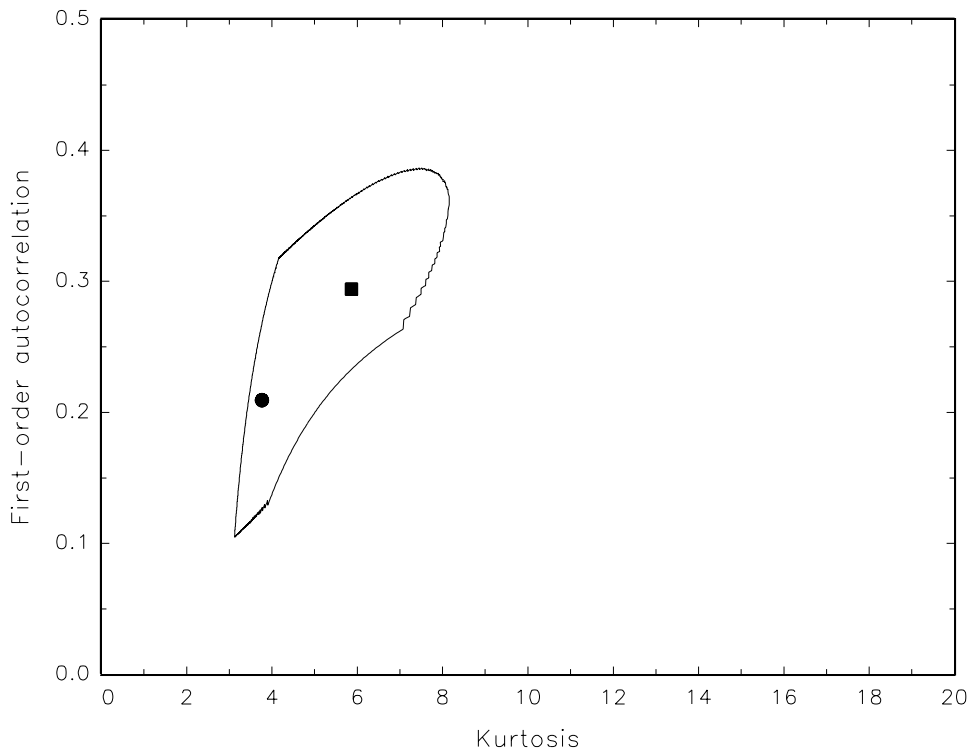
Figure 15: Approximate 90% confidence region based on 200 realizations of the true kurtosis/autocorrelation combination for the Assi D return series under the assumption that the observations have been generated by an EGARCH(1,1) model. Solid square is the nonparametrically estimated value, solid circle is the plug-in estimate.
