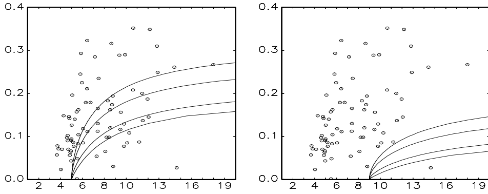
Figure 5: Combinations of the first-order autocorrelation of squared observations and kurtosis for the GARCH(1,1) model with t-distributed errors for various values of \alpha\nu_2 + \beta : left panel: t(7) , right panel: t(5) . Isoquants from lowest to highest: \alpha + \beta = 0.999, 0.99, 0.95 and 0.9 . The observed combinations are the same as in the lower-right panel of Figure 1.
