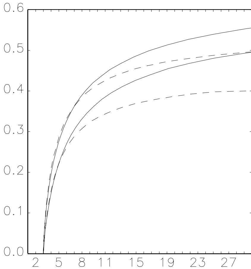
Figure 9: Combinations of two first-order autocorrelations, the squared observations (dashed line) and the absolute observations (solid line), and corresponding kurtosis values for the EGARCH(1,1) model with normal errors for \beta = 0.99 (low) and \beta = 0.95 (high).
