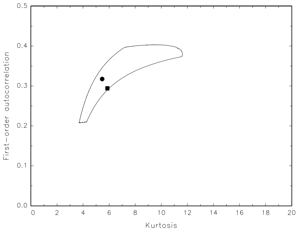
Figure 14: Approximate 90% confidence region based on 200 realizations of the true kurtosis/autocorrelation combination for the Assi D return series under the assumption that the observations have been generated by a GARCH(1,1) model. Solid square is the nonparametrically estimated value, solid circle is the plug-in estimate.
