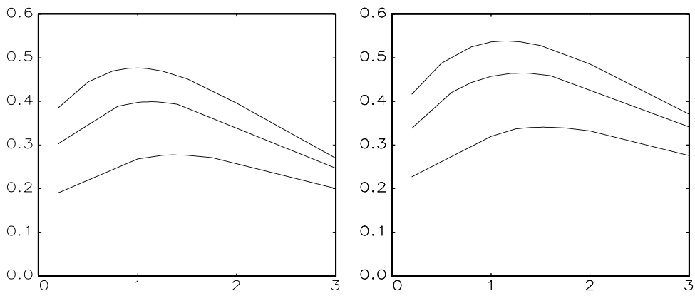
Figure 10: Combinations of the first-order autocorrelation of absolute-valued observations raised to power m as a function of m for the EGARCH(1,1) model with normal errors for \beta = 0.95 (left panel) and \beta = 0.99 (right panel) at three kurtosis values. From low to high: \kappa_4 = 6, 12 and 24 .
