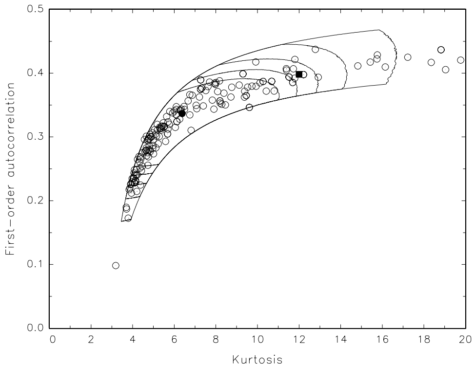
Figure 13: Simulated kurtosis/autocorrelation combinations for the GARCH(1,1) model with (\alpha_0, \alpha_1, \beta) = (0.05, 0.19121, 0.75879) , and approximate 50%, 60%, 70%, 80%, and 90% confidence intervals of the true value, 1000 observations and 200 realizations. Solid square is the true value; solid circle is the plug-in estimate; empty circles are generated combinations.
