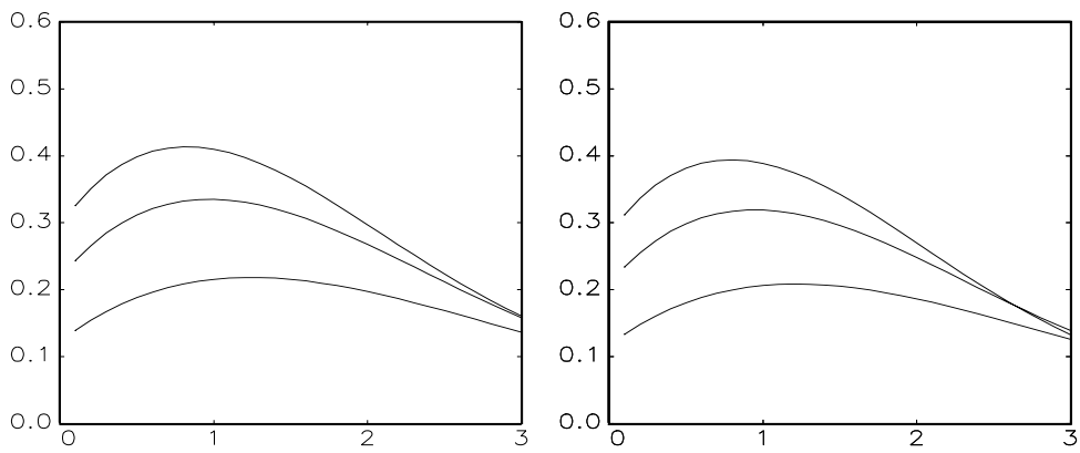
Figure 12: Combinations of the first-order autocorrelation of absolute-valued observations raised to power m as a function of m for the ARSV(1) model with normal errors for \beta = 0.95 (left panel) and \beta = 0.99 (right panel) at three kurtosis values. From low to high: \kappa_4 = 6, 12 and 24 .
