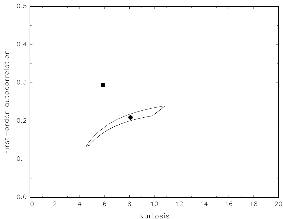
Figure 16: Approximate 90% confidence region based on 200 realizations of the true kurtosis/autocorrelation combination for the Assi D return series under the assumption that the observations have been generated by an ARSV(1,1) model. Solid square is the nonparametrically estimated value, solid circle is the plug-in estimate.
