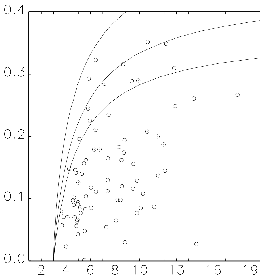
Figure 6: Combinations of the first-order autocorrelation of squared observations and kurtosis for the EGARCH(1,1) model with normal errors for various values of \beta . The isoquants from lowest to highest: \beta = 0.95, 0.99 and 0.999 . The observed combinations are the same as in the fourth panel of Figure 1.
