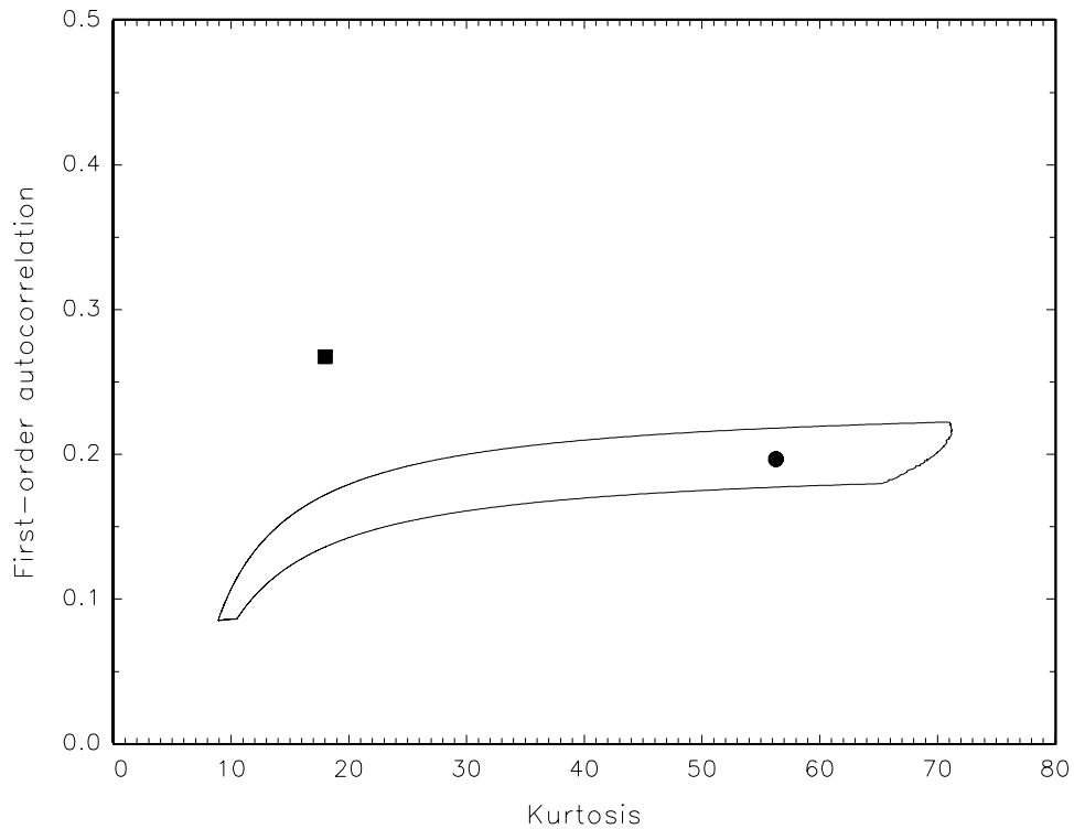
Figure 18: Approximate 90% confidence region based on 200 realizations of the true kurtosis/autocorrelation combination for the SEB return series under the assumption that the observations have been generated by a GARCH(1,1) model with t-distributed errors ( \nu = 7 ). Solid square is the nonparametrically estimated value, solid circle is the plug-in estimate.
