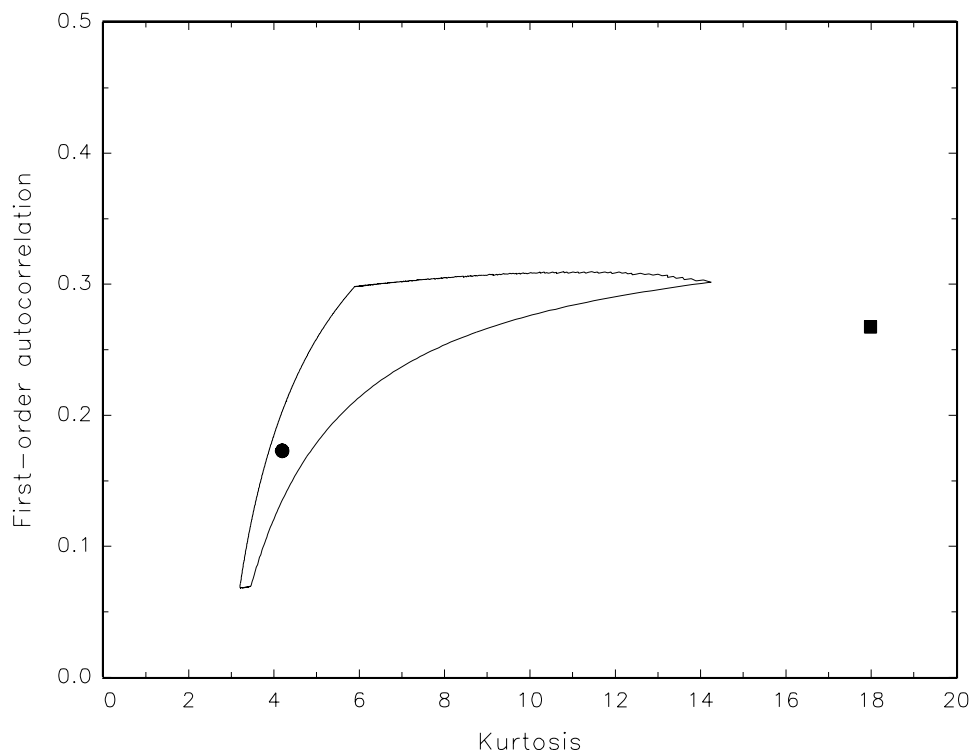
Figure 19: Approximate 90% confidence region based on 200 realizations of the true kurtosis/autocorrelation combination for the SEB return series under the assumption that the observations have been generated by an EGARCH(1,1) model. Solid square is the nonparametrically estimated value, solid circle is the plug-in estimate.
