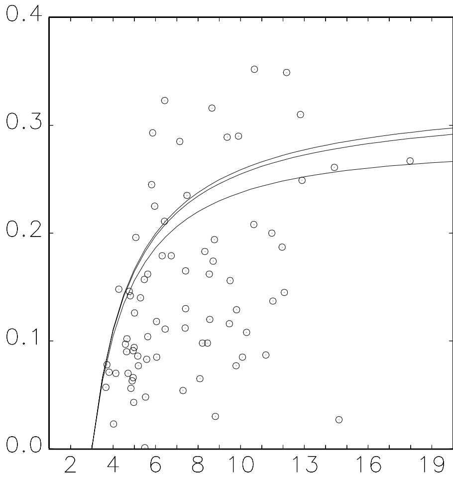
Figure 7: Combinations of the first-order autocorrelation of squared observations and kurtosis for the ARSV(1) model with normal errors for various values of \beta . Isoquants from lowest to highest: \beta = 0.999, 0.99 and 0.95 . The observed combinations are the same as in the lower-right panel of Figure 1.
