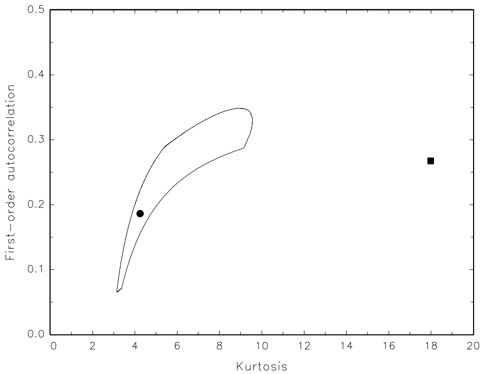
Figure 17: Approximate 90% confidence region based on 200 realizations of the true kurtosis/autocorrelation combination for the SEB return series under the assumption that the observations have been generated by a GARCH(1,1) model. Solid square is the nonparametrically estimated value, solid circle is the plug-in estimate.
