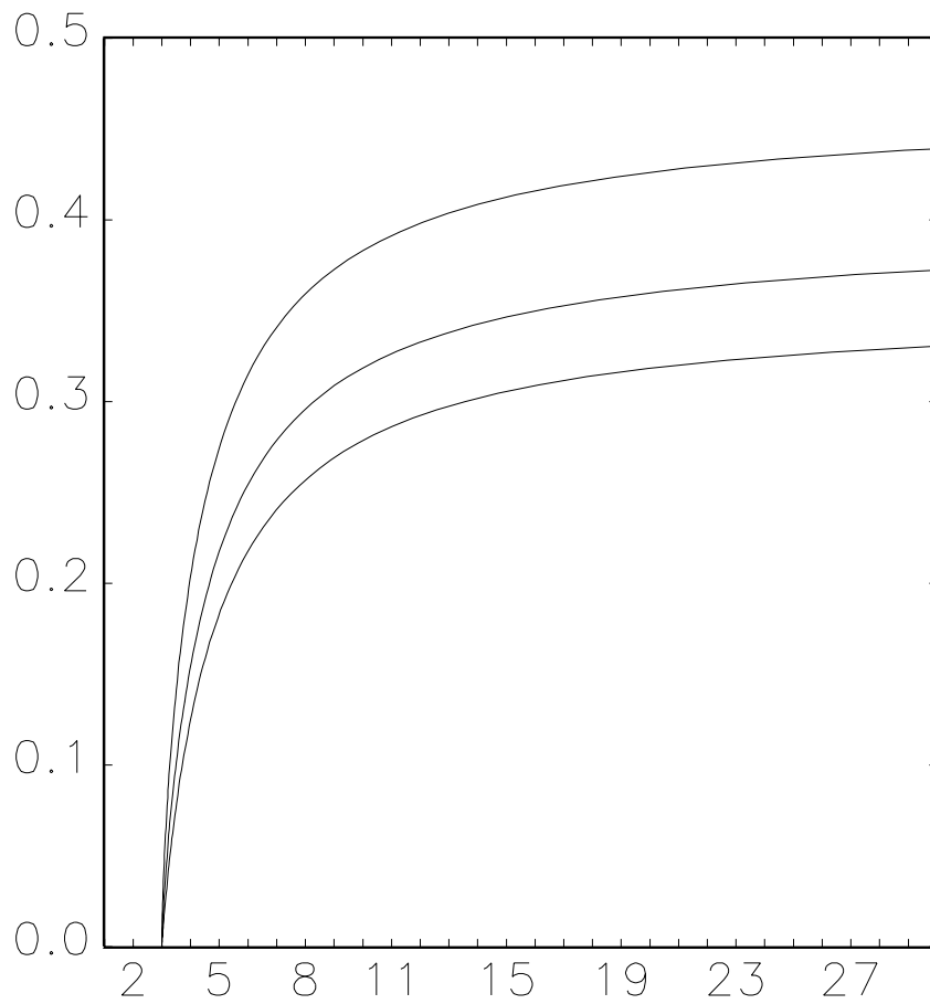
Figure 2: Combinations of the first-order autocorrelation of squared observations and kurtosis for the GARCH(1,1) model with normal errors for various values of \alpha + \beta . Isoquants from lowest to highest: \alpha + \beta = 0.999, 0.99 and 0.95 .
